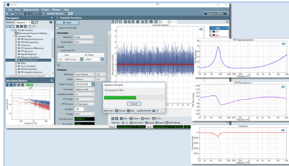
Example test results—impedance magnitude, phase and coherence—of a loudspeaker tested using a noise signal with the APx500 software’s transfer function measurement capability (v5.0 or later).
