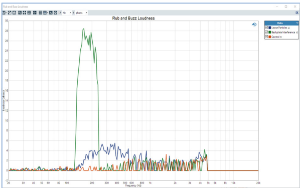
APx500 software (v6.1 or later) offers the broadest set of rub & buzz defect detection methodologies available to speaker designers and manufacturers: Rub & Buzz, SoneTrac, High-Order Harmonic Distortion (HOHD) and Rub & Buzz Loudness (shown above).
