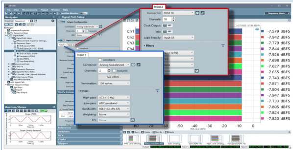
An illustration of the simultaneous multi-input capability of APx500 software, in this case an example application of 16 digital mics as the DUTs on Input 2 and an analog measurement mic as the reference on Input 1 (v6.0 or later).
