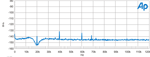
Figure 4. Typical residual THD+N spectrum at 20 kHz, 2 Vrms. (32768 point FFT of notch filter output, Sample Rate = 262 ks/s, 16 averages).
