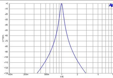
Figure 29. Digital Domain Bandpass filter response.
