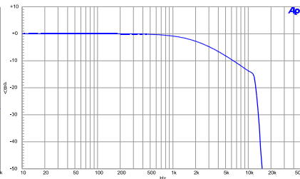
Figure 15. FIL-D75B.75 \mu s with 15.734 kHz (NTSC) notch De-emphasis Filter.
