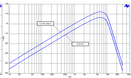
Figure 8. FIL-CCR. IEC468 (CCIR)/DIN 45404 Noise Weighting Filter.
