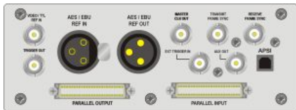
Figure 34. Miscellaneous digital I/O Panel (rear of SYS-2720 and SYS-2722 instruments only).
