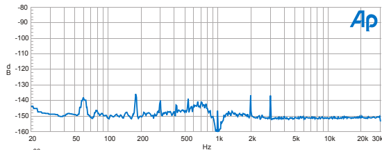
Figure 3. Typical residual THD+N spectrum at 1 kHz, 2 Vrms. (32768 point FFT of notch filter output, Sample Rate = 65.536 ks/s, 16 averages).
