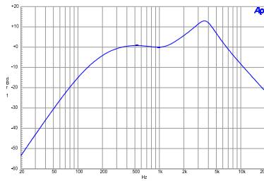
Figure 28. Digital Analyzer F-weighting curve.
