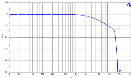
Figure 13. FIL-D50F.50 \mu s with 19 kHz (FM) notch De-emphasis Filter.
