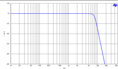
Figure 19. 8 kHz 7-pole Low Pass Filter.
