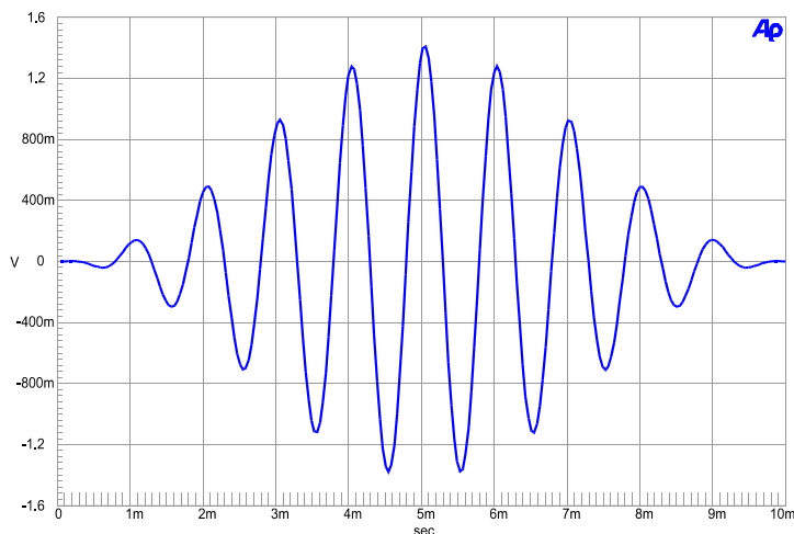
Figure 30. Shaped Sine Burst signal. (1 kHz, 10 cycles)
