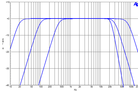
Figure 6. Typical responses of the standard band-limiting filters.
