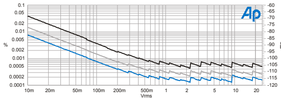
Figure 2. Typical system THD+N versus amplitude at 1 kHz. Lower trace is with 22 kHz bandwidth limiting. Middle trace is with 80 kHz.
