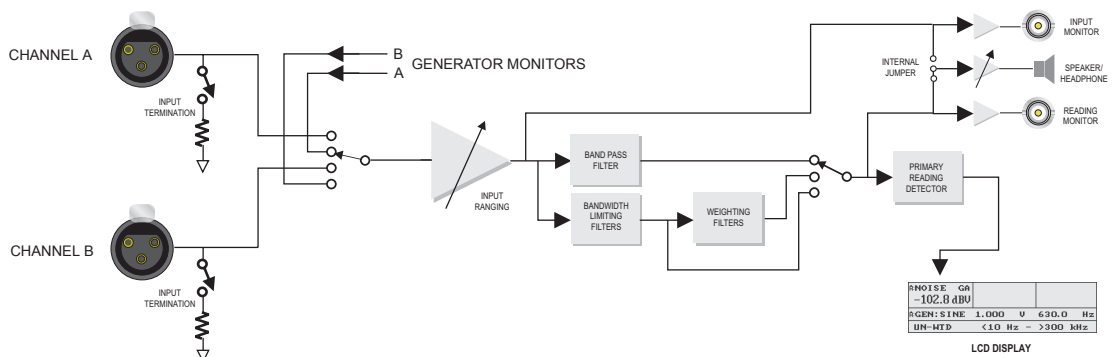
Figure 4-4. Block Diagram of Analog NOISE Measurement
