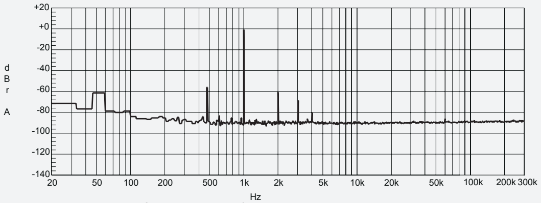
Figure 4-11. Spectrum with no filter
