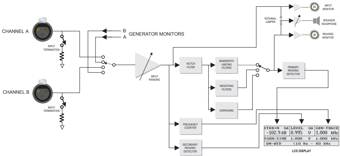
Figure 4-8. Block Diagram of Analog THD+N Measurement
