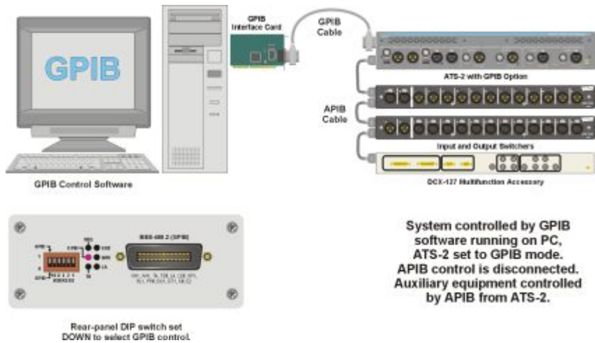
Figure 27. APIB connections to ATS-2 with GPIB option in GPIB control mode. SWR-2122 Switcher and DCX-127 connected to the APIB connector of the ATS-2. The computer APIB cable is not connected.
