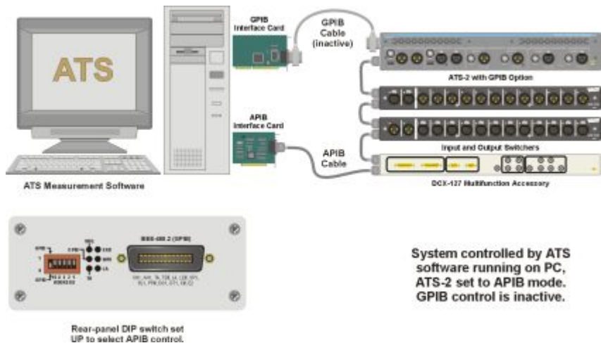
Figure 28. APIB controller connections, ATS-2 with GPIB option in APIB control mode. Computer APIB cable connected to DCX-127, then to SWR-2122, then to ATS-2.
