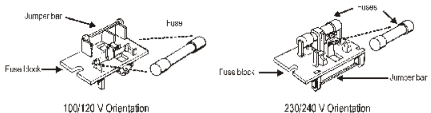
Figure 6. Fuse Block Orientation for North American (100/120 V) and European (230/240 V) operation..
